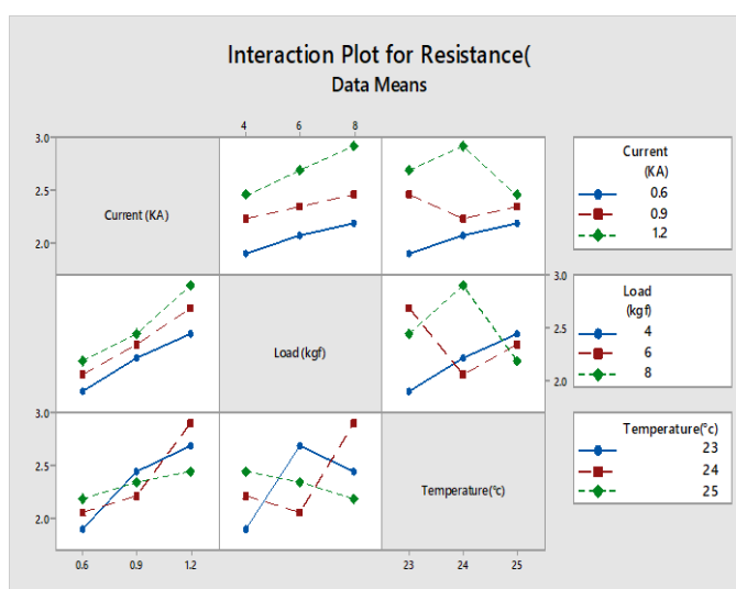
Figure 5: Interaction Plots
