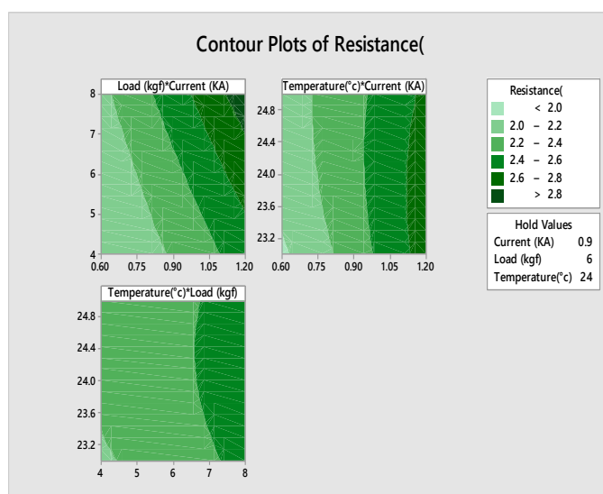
Figure 6: Contour Plots
