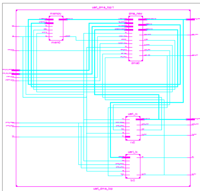
Fig 8: RTL schematic
