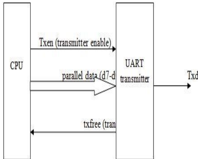
Fig2. UART transmitter
