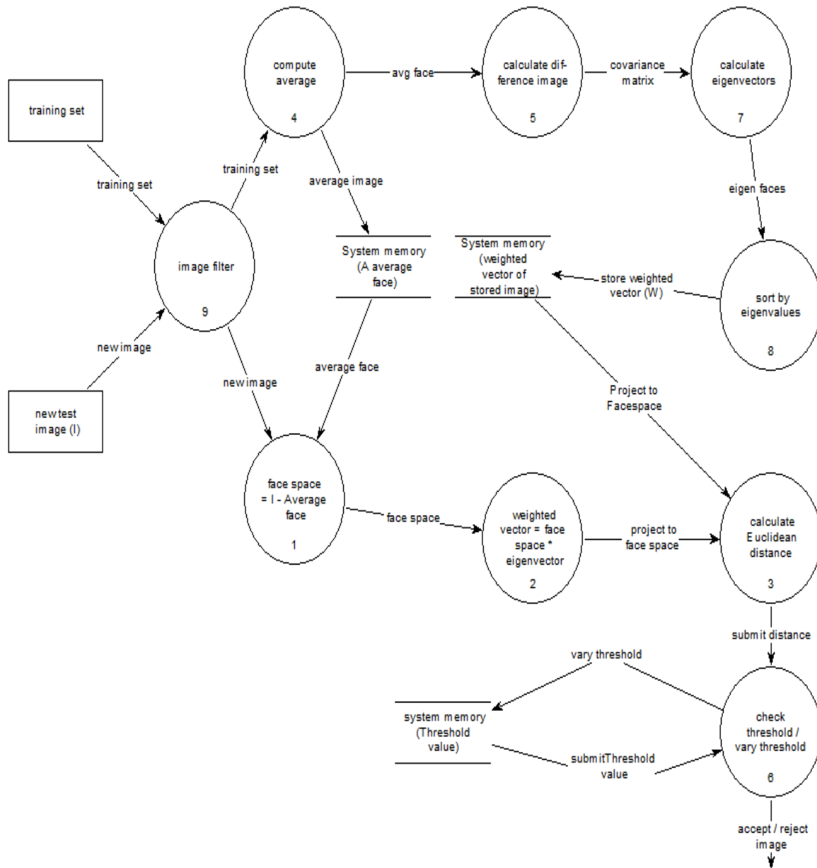
Figure: Behavioural model for Eigenface Recognition System
