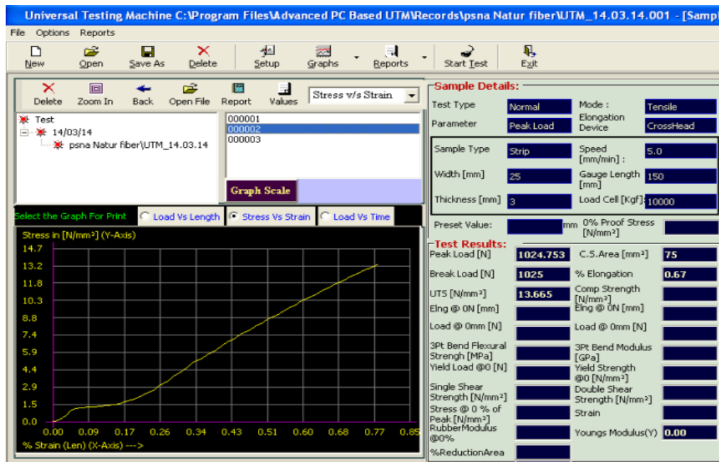
Figure 2B: Stress vs Strain
