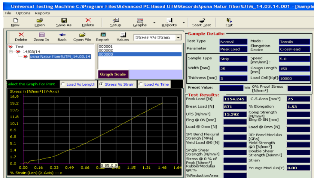
Figure 2C: Stress vs Strain
