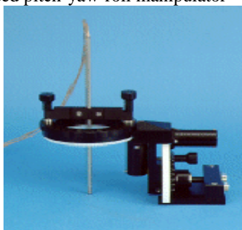
Fig 2 Dantec Dynamics motorised calibrator
