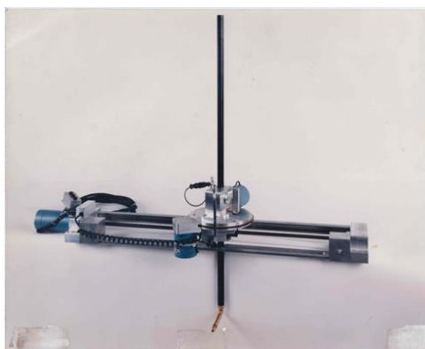
Fig 4 Aerolab Probe Traverse mechanism
