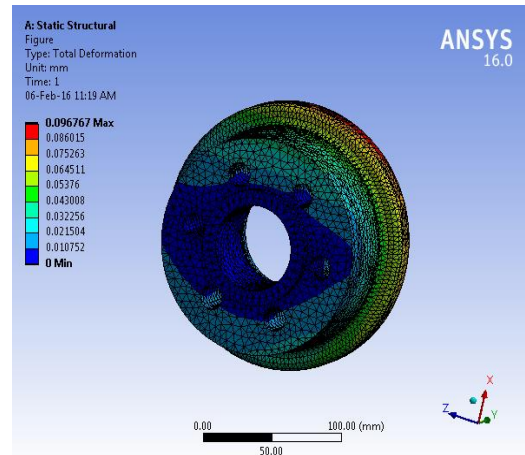
Fig.9 Deformation of wheel hub
