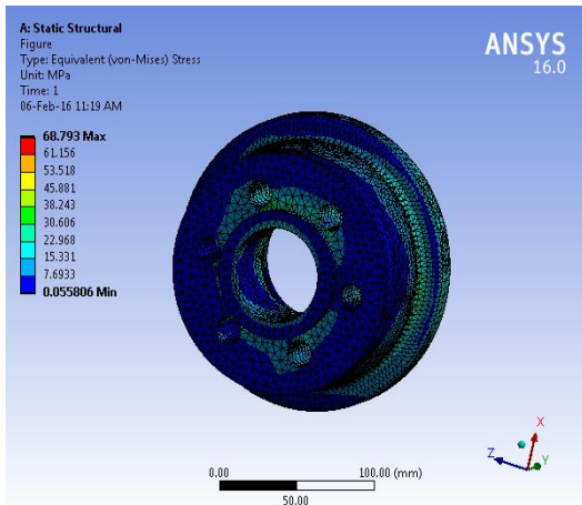
Fig.8 von-Mises stress at the wheel hub
